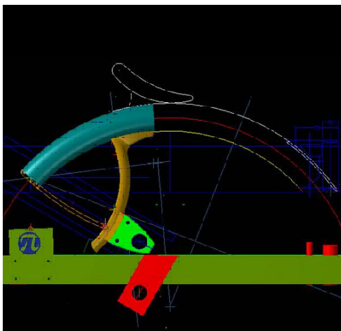
PiMoto aluminum monocoque in fixture drawing. Image courtesy of Pi Mobility.
